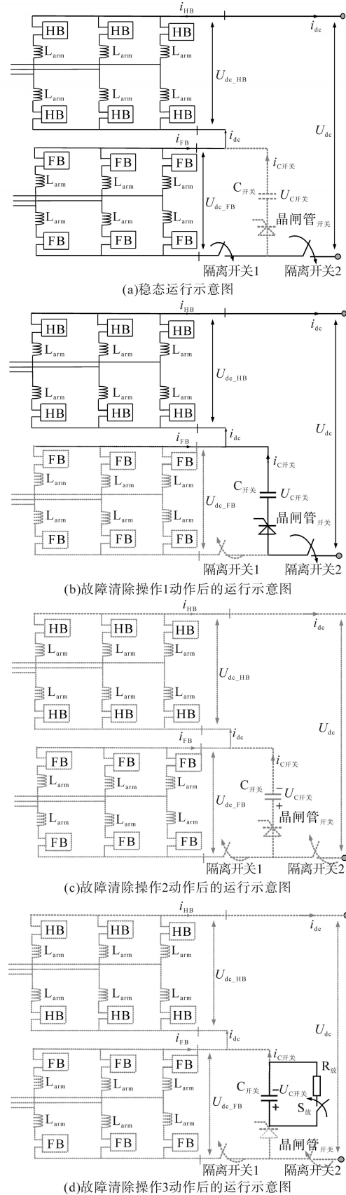
图2 不同状态下的TSC-hybrid MMC运行示意图 Fig.2 Schematic of TSC-hybrid MMC at different operating states TSC-hybrid MMC的稳态状态如图2a所示,
